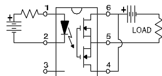
"C" Connection
